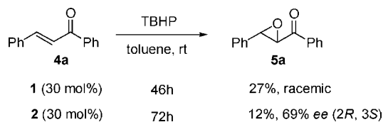
Scheme 1. Epoxidation of trans -Chalcone 4a by Catalysts 1 and 2
