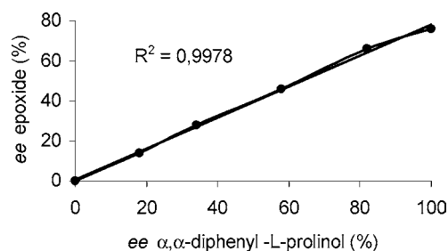
Figure 2. Linear effect in the \alpha,\alpha -diphenyl-L-prolinol-mediated epoxidation of chalcone 4a . R = correlation coefficient.
