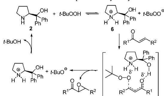
Scheme 2. Proposed Catalytic Cycle
